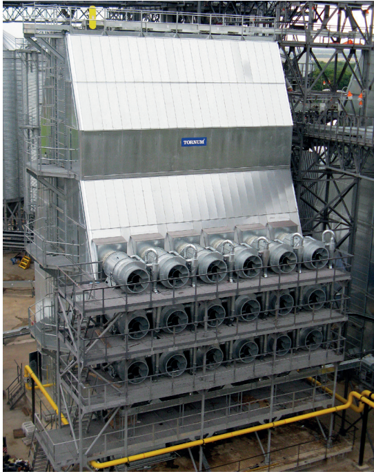
Tornum TK BIG dryer installed in Zhmerynka, Ukraine.
